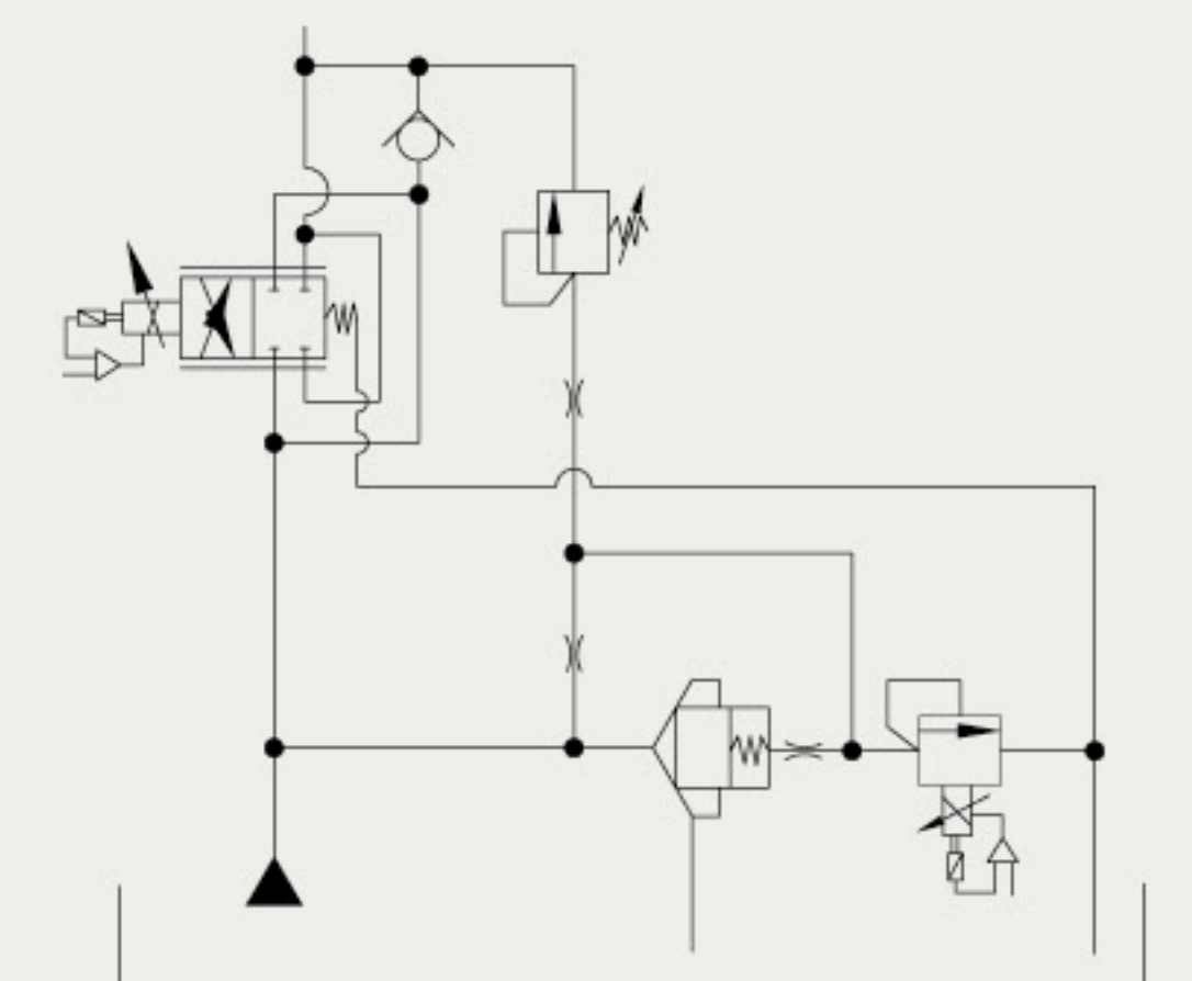
注塑机液压系统闭环反馈控制原理图 injection molding machine hydraulic system closed-loop feedback control schematics
